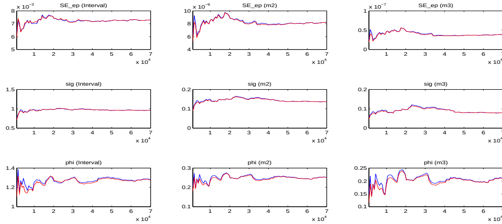
Figure 9: Gelman-Brooke Test
