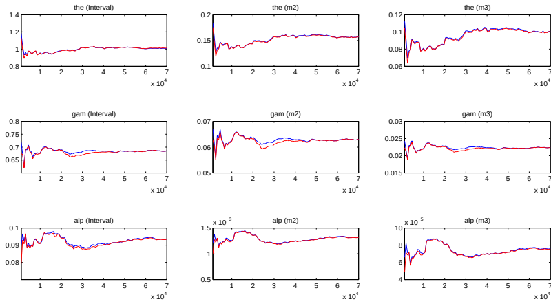
Figure 10: Gelman-Brooke Test
