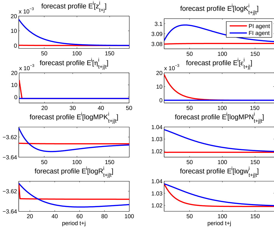
Figure 10: Impulse response in PI economy (2)
