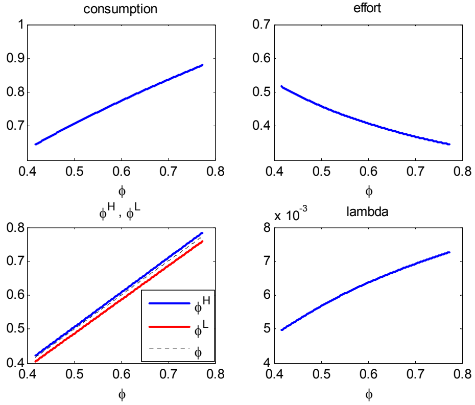
Figure 1: Policy functions: consumption, effort, Pareto weights and ICC Lagrange multiplier
