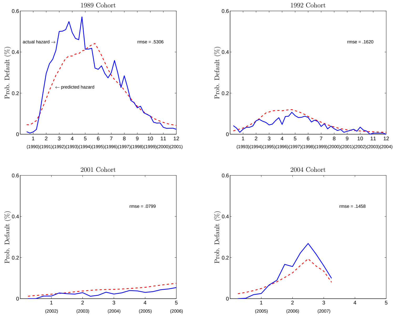
Figure 13: Predicted versus Actual Default Hazard Rates
