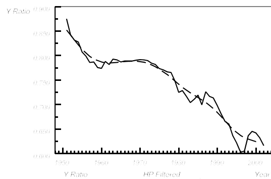
Fig. 6: Ratio of actual Y to counterfactual Y|_{R=R(1949)}
