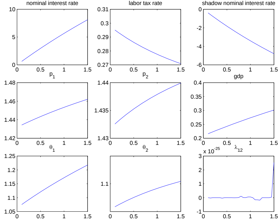
Figure 7: Steady-state Ramsey policy and allocation variables as function of importance of search goods, governed by \vartheta .
