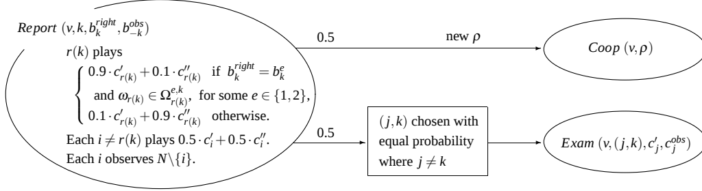
Figure 5: Report states
