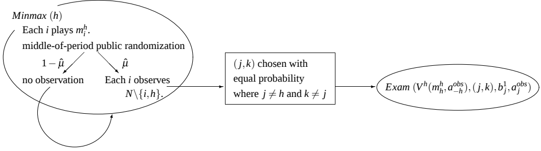
Figure 6: Minmax states
