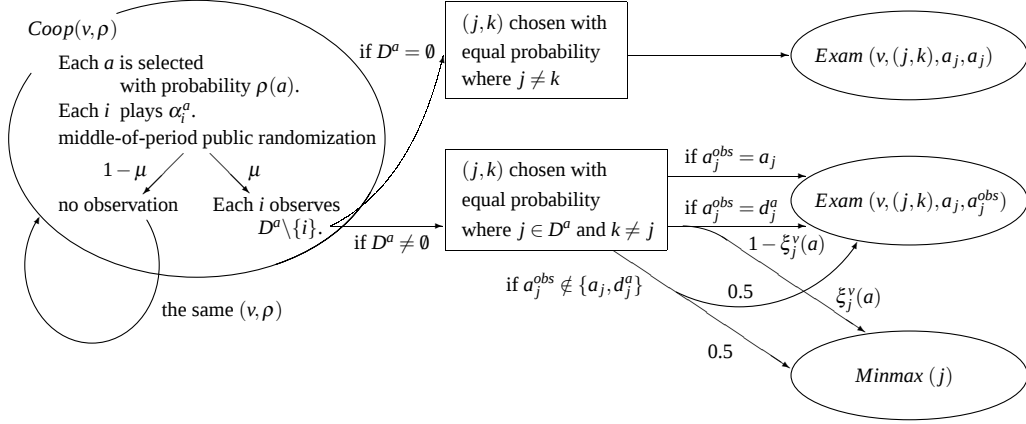
Figure 3: Cooperation states
