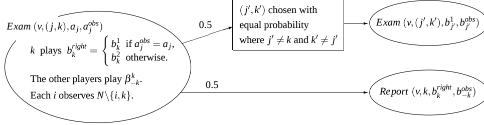
Figure 4: Examination states
