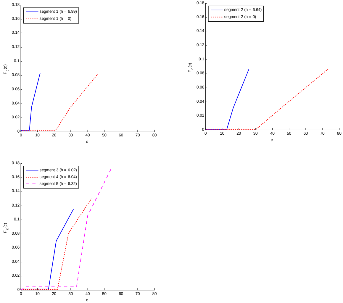
Figure 4: Estimated search cost distributions
