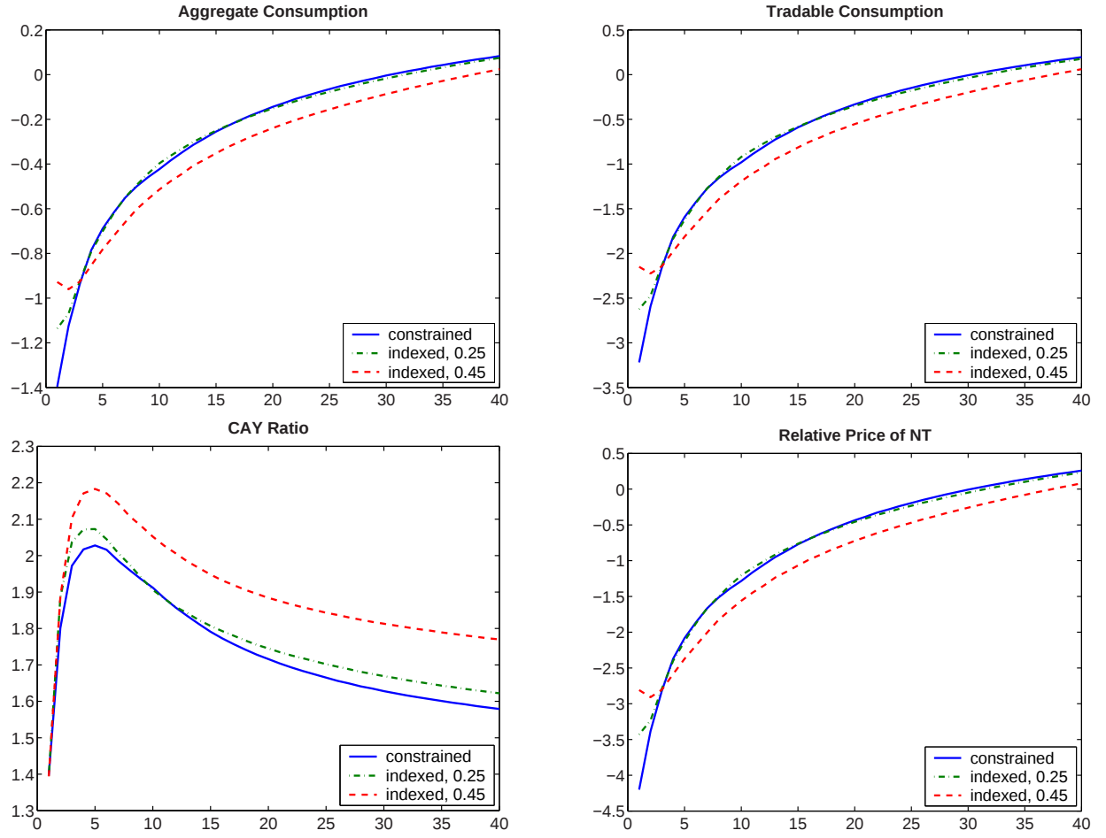
Figure 6: Conditional Forecasting Functions in Response to a 1-Standard-Deviation Negative Endowment Shock
