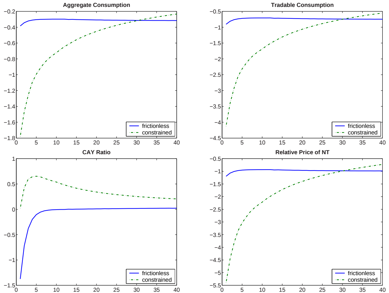
Figure 4: Conditional Forecasting Functions in Response to a 1-Standard-Deviation Negative Endowment Shock
