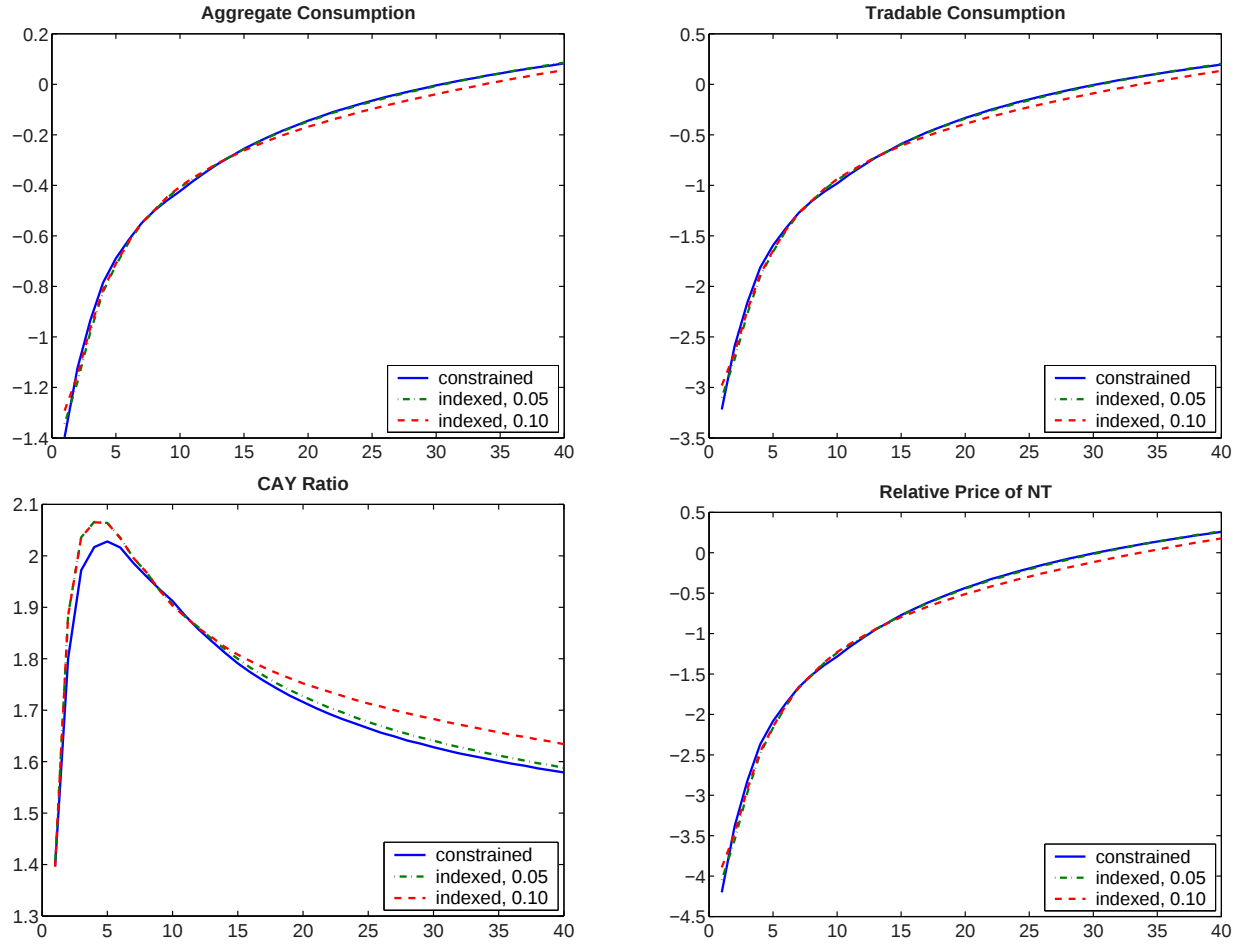
Figure 5: Conditional Forecasting Functions in Response to a 1-Standard-Deviation Negative Endowment Shock
