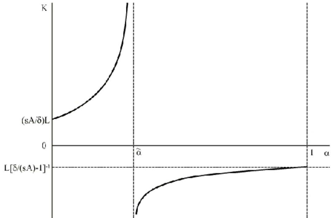
Figure 6: Unconstrained stationarity locus
