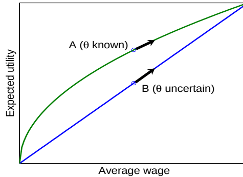
Figure 3: UNCERTAINTY AMPLIFIES THE MARGINAL UTILITY EFFECT OF A WAGE INCREASE. A is the utility of the agent who is certain about the value of nurture. B is the expected utility of the uncertain agent. The slope at A is smaller than the slope at B.
