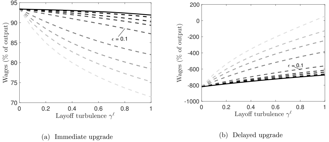
Figure C.4: AVERAGE WAGE IN PERIOD OF SKILL UPGRADE
