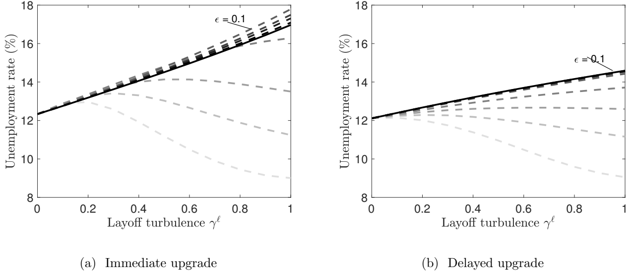
Figure C.3: TIMING OF COMPLETION OF SKILL UPGRADE IN BENCHMARK WITH LS PROD.
