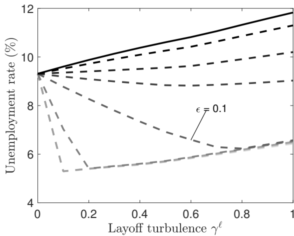
Figure D.4: DHHR vs. LS PRODUCTIVITY DISTRIBUTIONS IN DHHR MODEL
