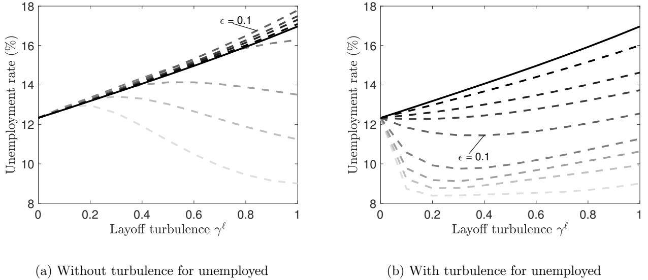
Figure E.1: TURBULENCE FOR UNEMPLOYED IN BENCHMARK WITH LS PRODUCTIVITY
